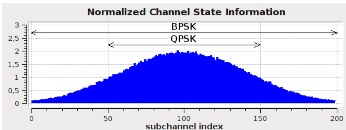
Figure 6.1: Using all subcarriers with BPSK and using the better half with QPSK
